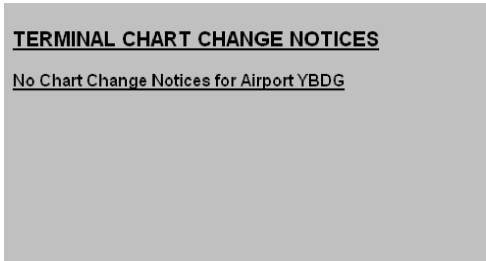
FIGURE 8: When no notice is available
